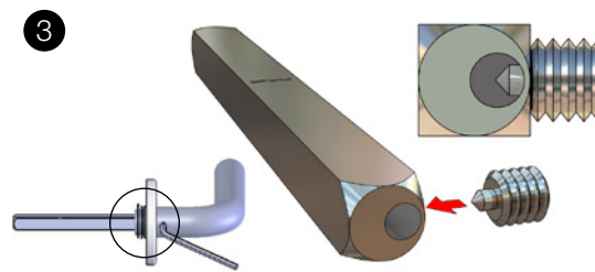
Complete handle with shaft Screw set 61 Tools for mounting
